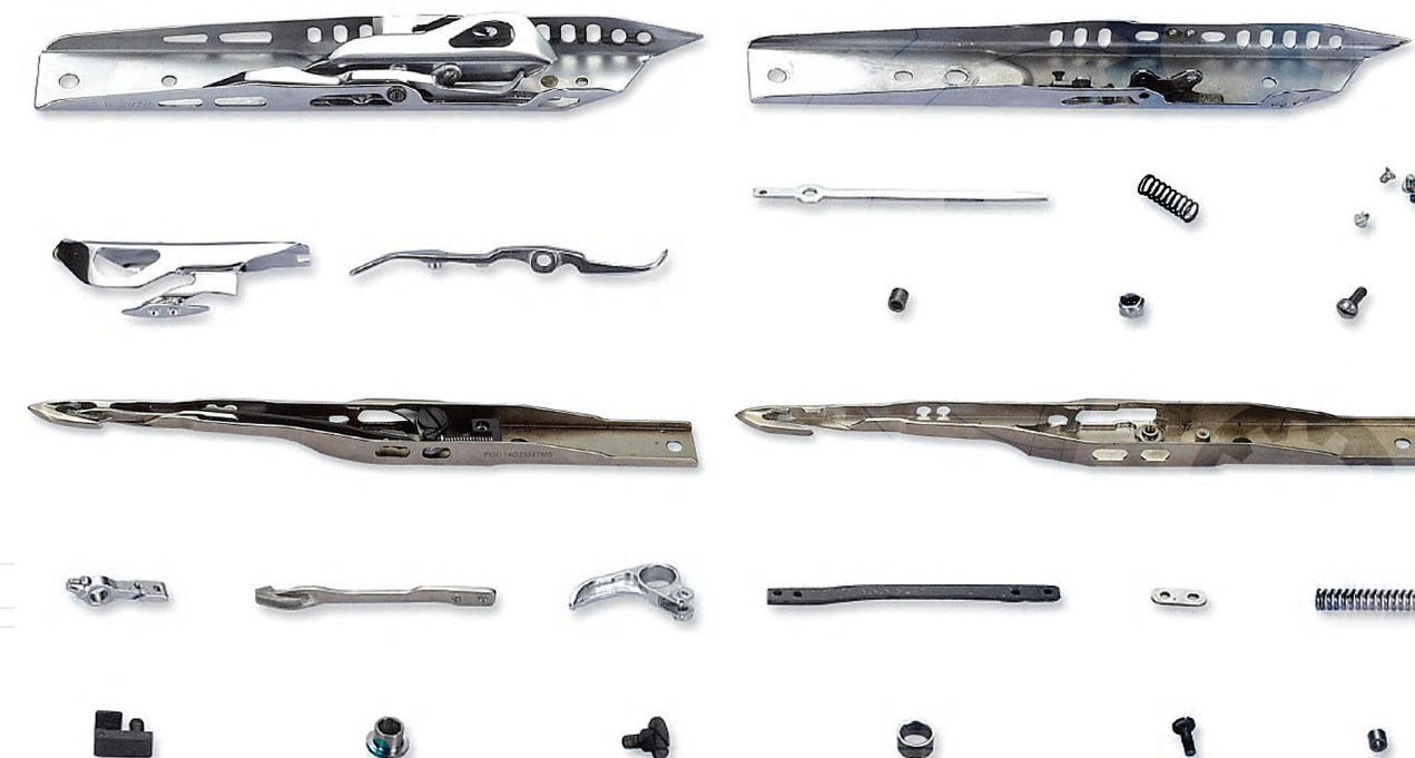
GS900 Rapier Gripper
