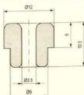
Eyelets / 瓷眼
