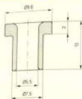
Eyelets / 瓷眼
