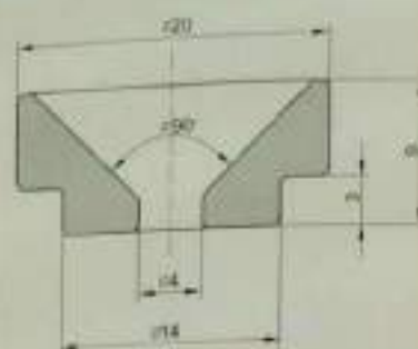
Eyelets / 瓷眼
