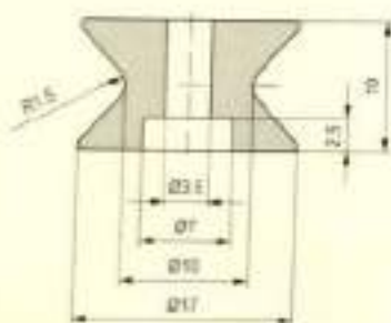
Rollers / 瓷轮
