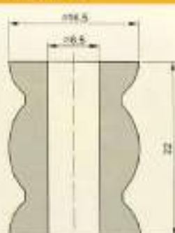
Rollers / 瓷轮
