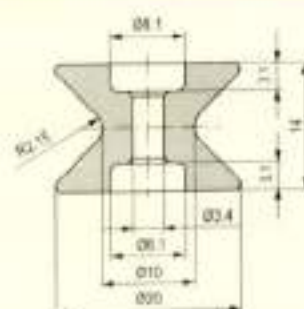
Rollers / 瓷轮
