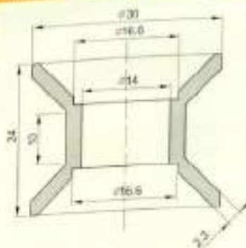
Rollers / 瓷轮
