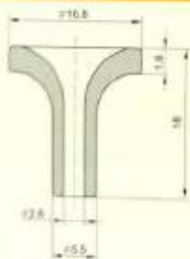
Eyelets / 瓷眼
