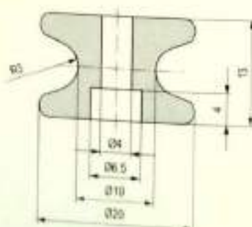
Rollers / 瓷轮
