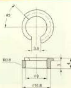
Eyelets / 瓷眼
