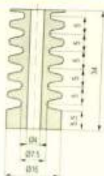
Rollers / 瓷轮
