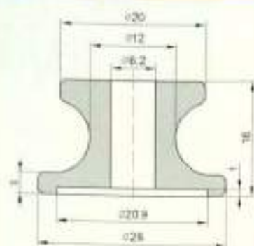
Rollers / 瓷轮
