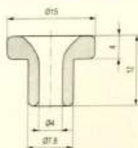
Eyelets / 瓷眼
