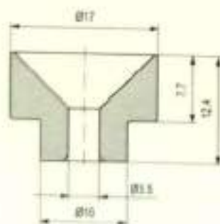
Eyelets / 瓷眼
