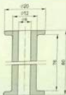
Rollers / 瓷轮
