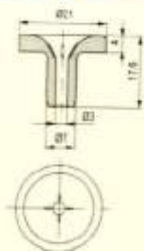
Eyelets / 瓷眼
