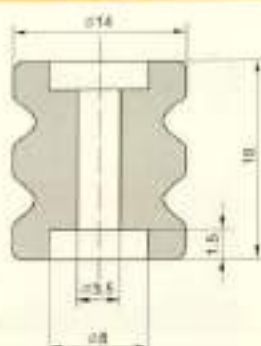
Rollers / 瓷轮
