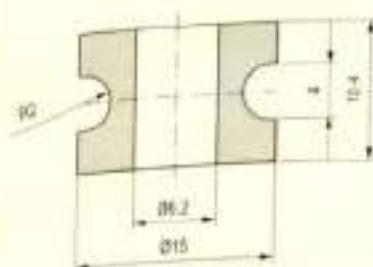
Rollers / 瓷轮
