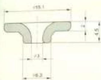
Eyelets / 瓷眼
