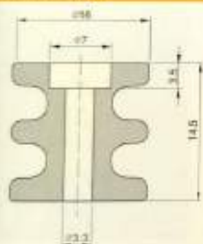
Rollers / 瓷轮
