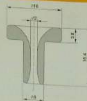
Eyelets / 瓷眼
