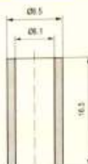
Tubes / 瓷管
