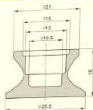
Rollers / 瓷轮
