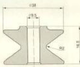
Rollers / 瓷轮
