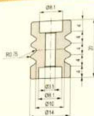
Rollers / 瓷轮
