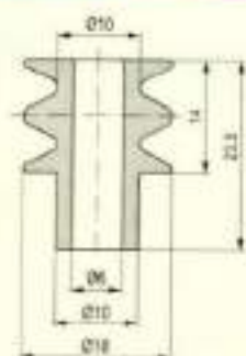
Rollers / 瓷轮
