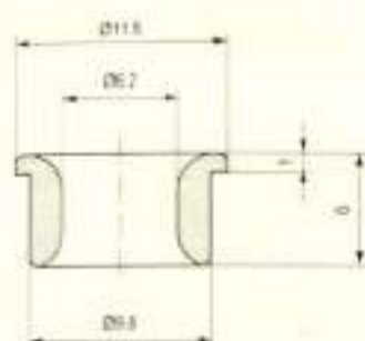
Eyelets / 瓷眼
