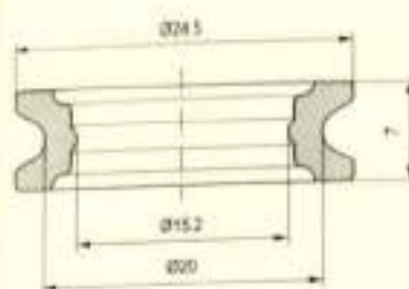
Eyelets / 瓷眼
