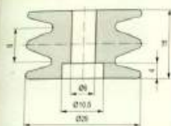
Rollers / 瓷轮
