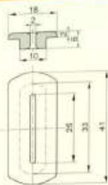
Eyelets / 瓷眼
