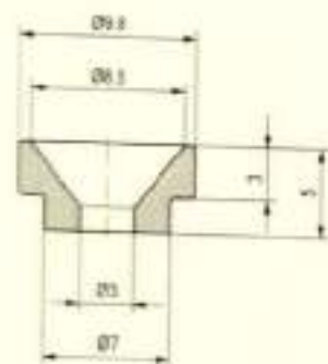
Eyelets / 瓷眼
