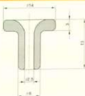
Eyelets / 瓷眼
