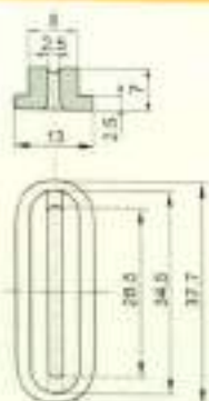
Eyelets / 瓷眼
