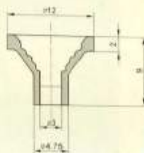
Eyelets / 瓷眼
