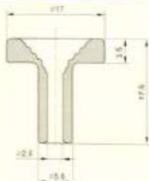
Eyelets / 瓷眼
