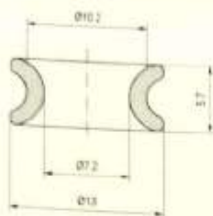
Eyelets / 瓷眼
