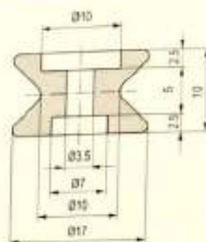
Rollers / 瓷轮
