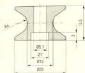
Rollers / 瓷轮
