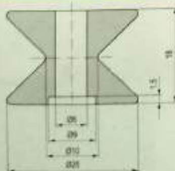
Rollers / 瓷轮
