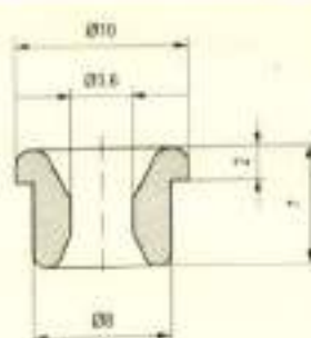
Eyelets / 瓷眼
