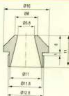
Eyelets / 瓷眼
