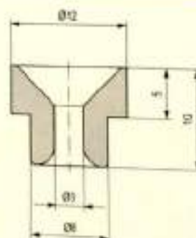
Eyelets / 瓷眼
