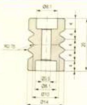
Rollers / 瓷轮
