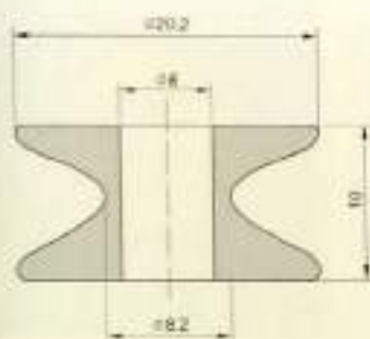
Rollers / 瓷轮
