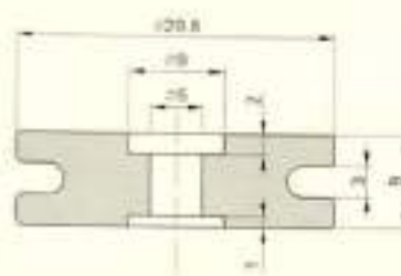
Rollers / 瓷轮
