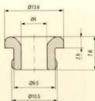
Eyelets / 瓷眼
