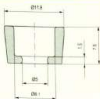
Eyelets / 瓷眼
