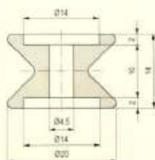
Rollers / 瓷轮
