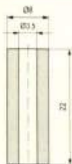
Tubes / 瓷管
