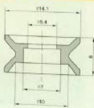
Rollers / 瓷轮
