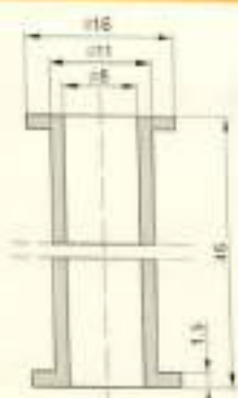
Rollers / 瓷轮
