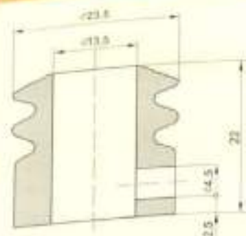
Rollers / 瓷轮
