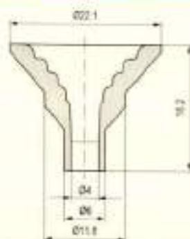
Eyelets / 瓷眼
