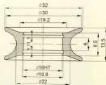
Rollers / 瓷轮
