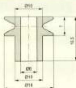
Rollers / 瓷轮
