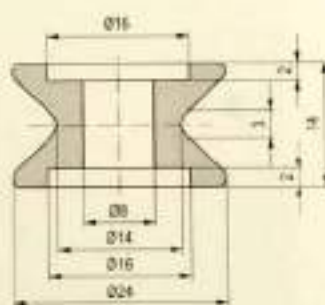
Rollers / 瓷轮
