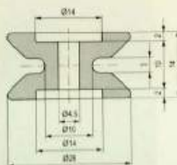
Rollers / 瓷轮
