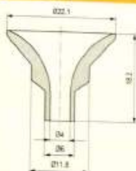
Eyelets / 瓷眼
