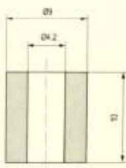
Tubes / 瓷管
