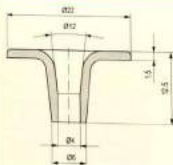
Eyelets / 瓷眼
