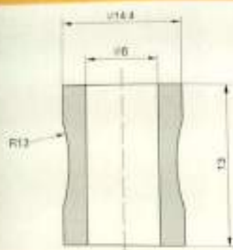
Rollers / 瓷轮
