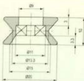
Rollers / 瓷轮
