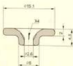
Eyelets / 瓷眼
