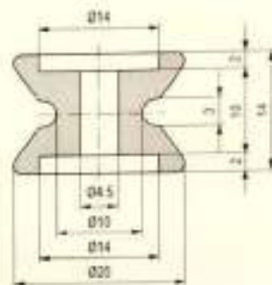
Rollers / 瓷轮
